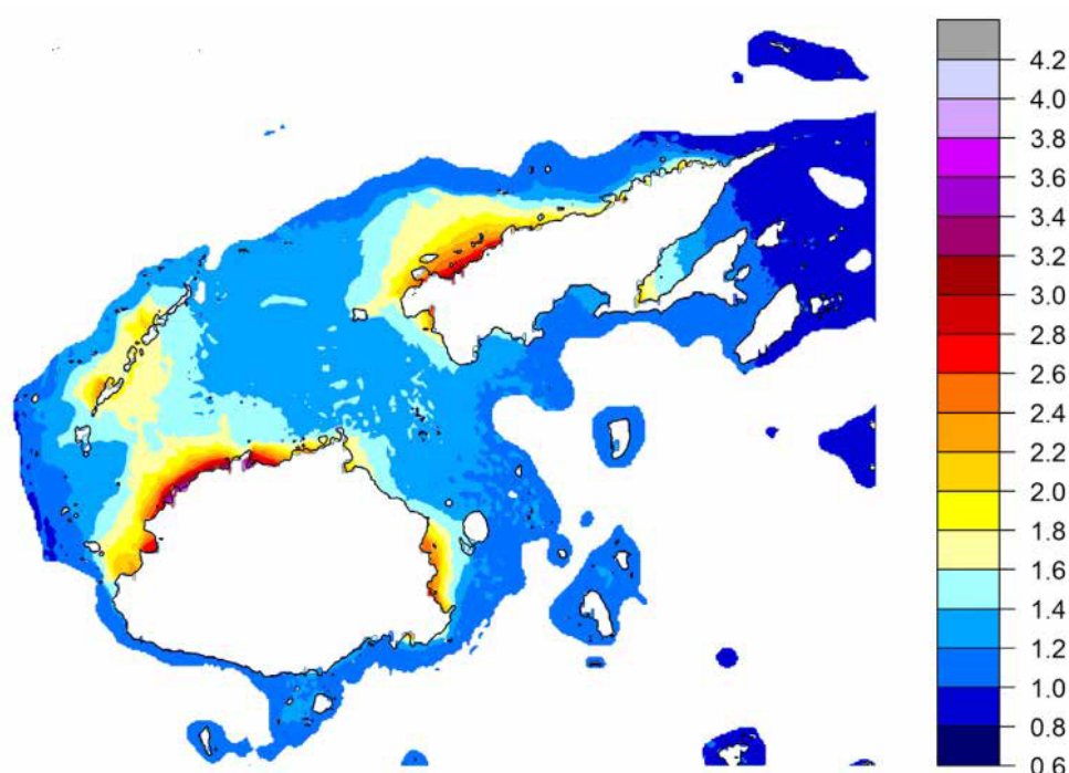
Figure 9: Maximum Modelled Storm Tide Heights in Fiji for 200-Year Annual Recurrence Interval Events (metres above MSL)
