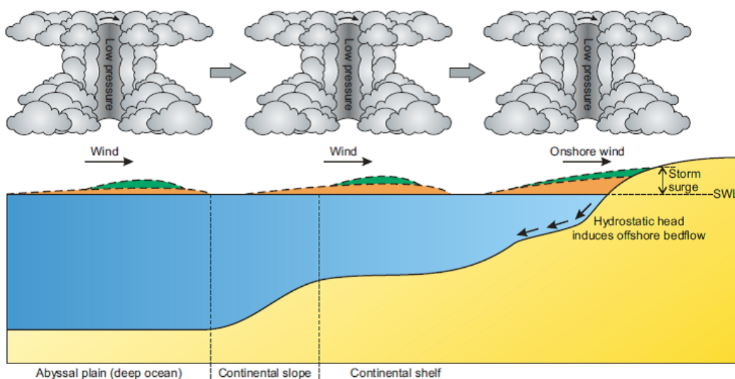
Figure 8: Processes Contributing to Storm Surge
