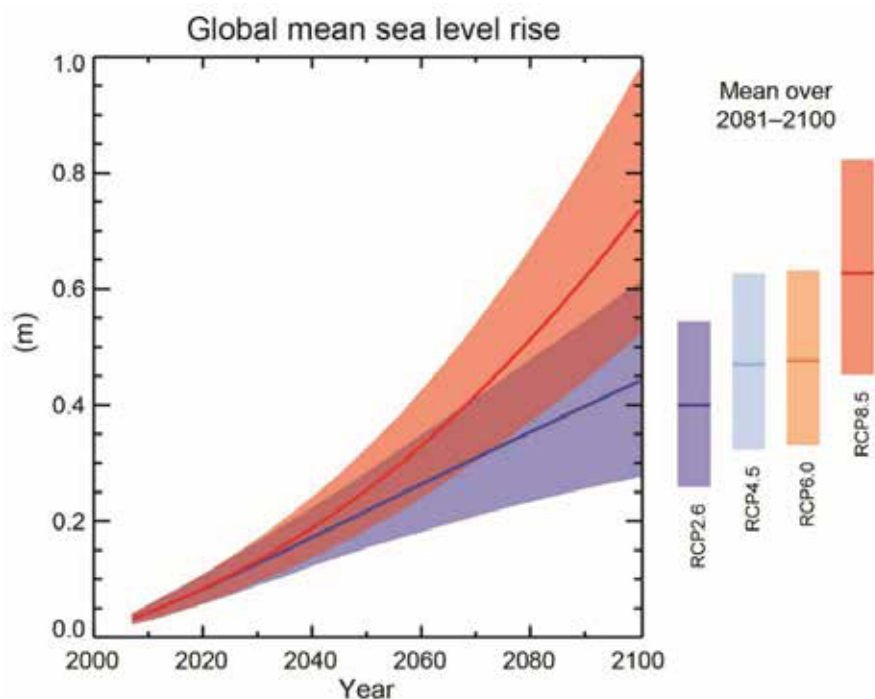
Figure 10: Projections of Potential Future Sea Level Rise Presented within the Fifth Assessment Report of the Intergovernmental Panel on Climate Change
