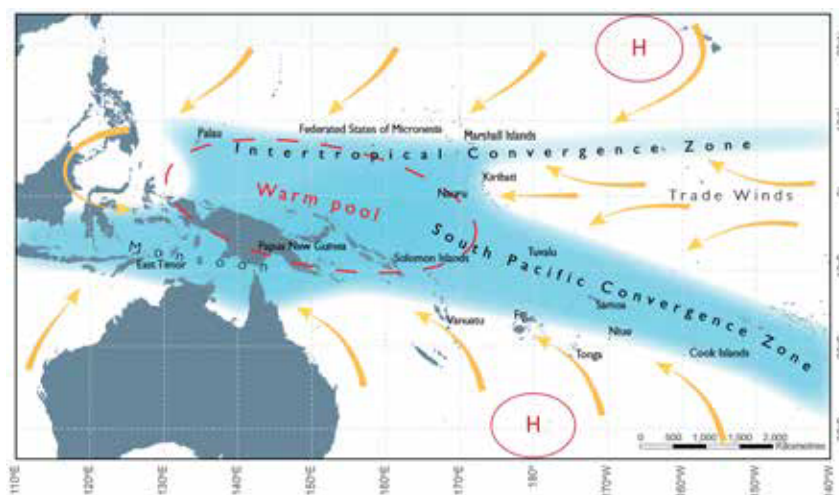
Figure 3: Average Positions of the Major Climate Features in the Southwest Pacific between November and April
